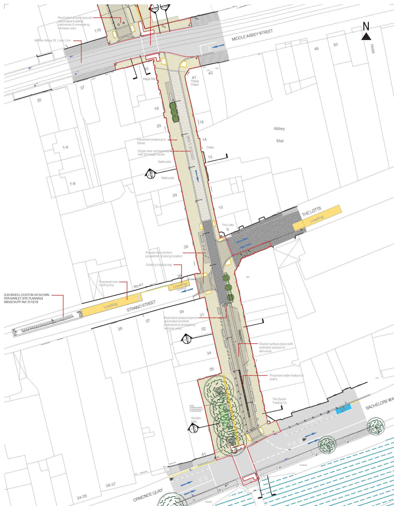
vi Liffey Street Lower Proposed Site Plan. See draft planning drawing dPL-109.
